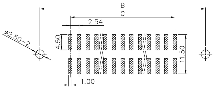
FBL layout (Top View)
