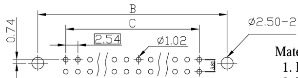
PCB Layout (Top View)
