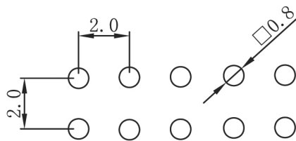
P. C. B Hole Layout
