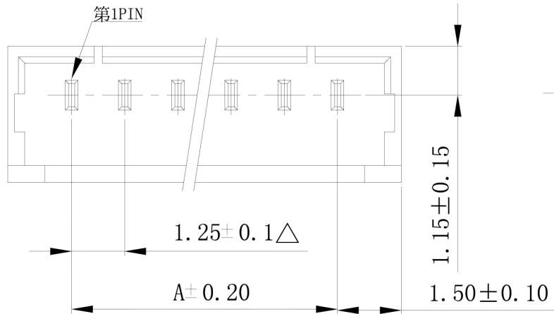
P. C. B Hole Layout
