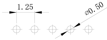
P. C. B Hole Layout
