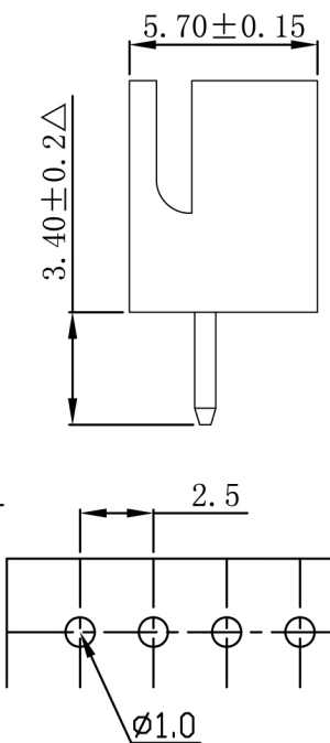
P. C. B Hole Layout
